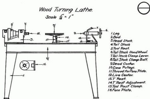
Fig. 1. - Wood Turning Lathe
