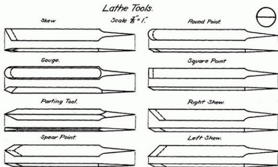
Fig. 2. - Lathe Tools
