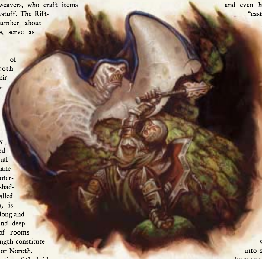
Cloaker attack
