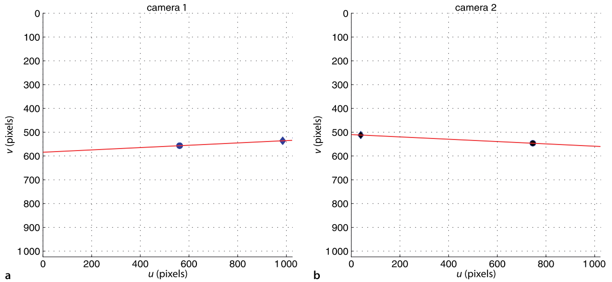
Fig. 14.7. Epipolar geometry simulation showing the virtual image planes of two Toolbox CentralCamera objects. The perspective projection of point P is a black circle, the projection of the other camera's centre is a black ♦-marker, and the epipolar line is shown in red
