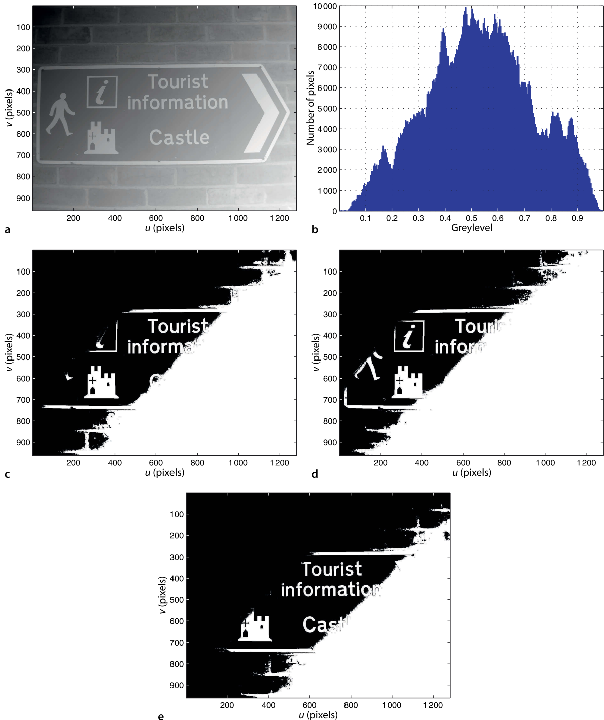
Fig. 13.3. Binary segmentation example. a Grey scale image with diagonal intensity gradient, b histogram, c thresholded with Otsu's threshold at 0.54, d thresholded at 0.50, e thresholded at 0.60
