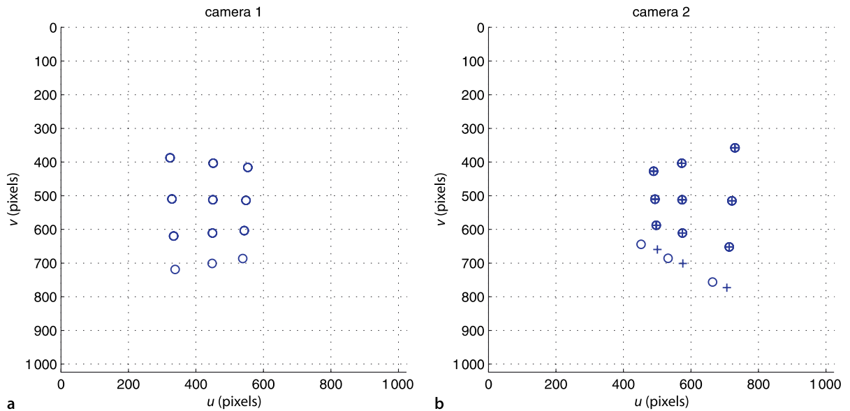
Fig. 14.13. Views of the oblique planar grid of points from two different view points. The grid points are projected as open circles. Plus signs in b indicate points transformed from the camera one image plane by the homography. The bottom row of points in each case are not co-planar with the other points
