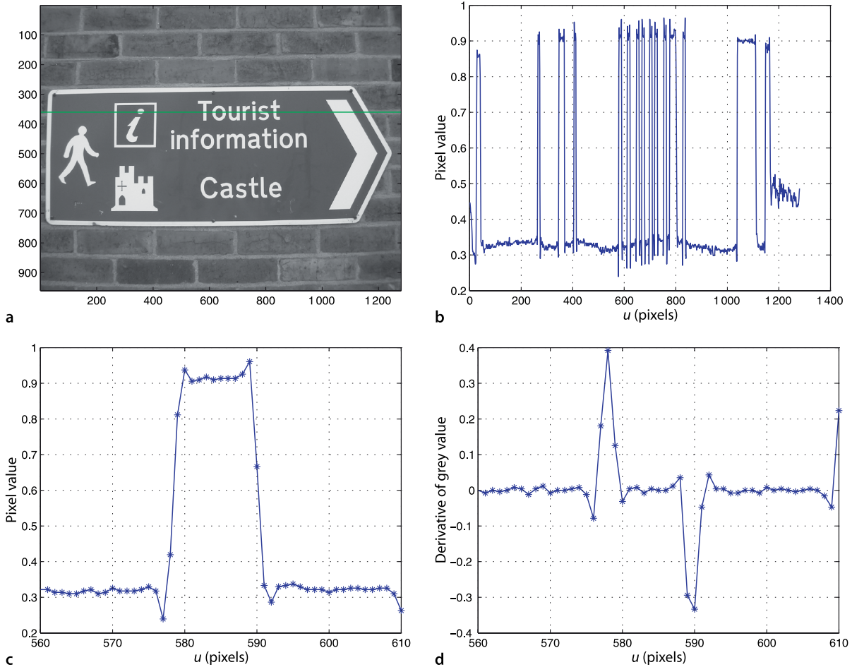
Fig. 12.15. Edge intensity profile. a Original image; b greylevel profile along horizontal line v = 360 ; c close up view of the spike at u \approx 580 ; d derivative of c (image from the ICDAR 2005 OCR dataset; Lucas 2005)
