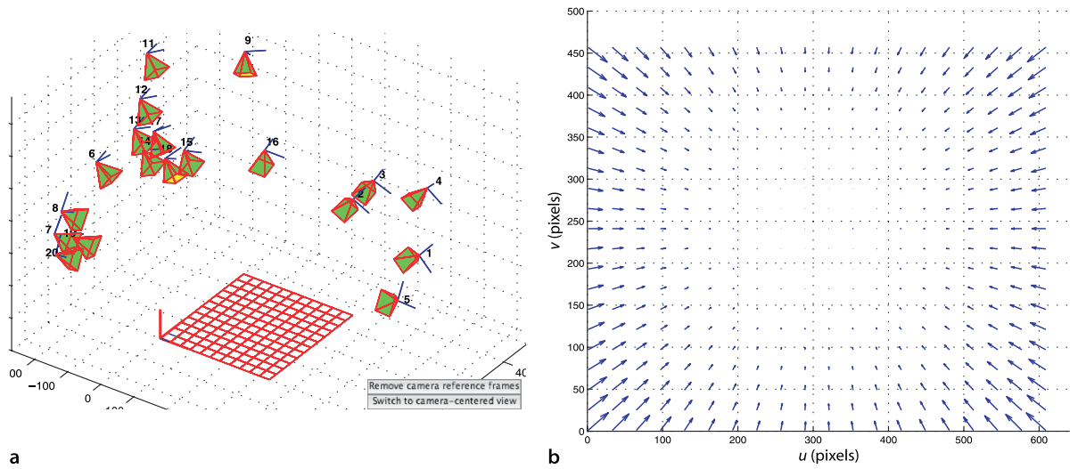
Fig. 11.12. Calibration results from the example in Bouguet's Calibration Toolbox. a The estimated camera pose relative to the target for each calibration image, b the distortion map with vectors showing how points in the image will move due to distortion
