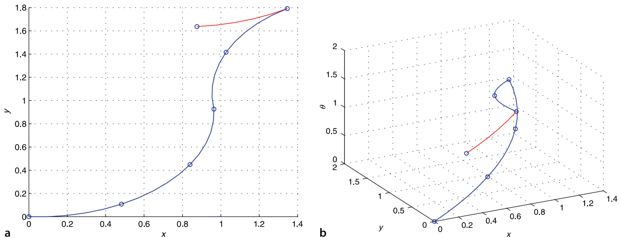
Fig. 5.14. The path computed by RRT that translates the non-holonomic vehicle sideways. Nodes in the RRT are shown as circles , forward motion is shown in blue , reverse motion in red . a Path in the xy -plane; b path in the (x, y, \theta) space
