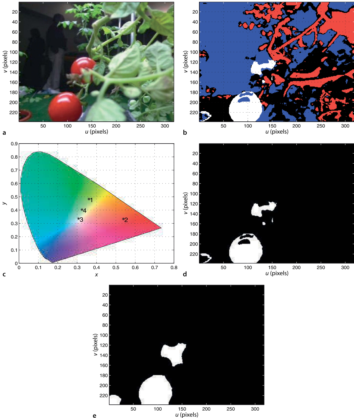
Fig. 13.7. Garden image example. a Original image (courtesy of Distributed Robot Garden project, MIT); b pixel classification ( C=4 ) shown in false color; c cluster centres in the xy -chromaticity space; d all pixels of class c=2 ; e after morphological closing with a circular structuring element of radius 15
